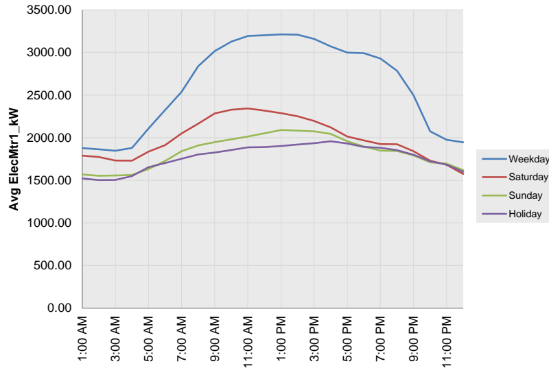
Figure 4: Main Campus Demand Loads
