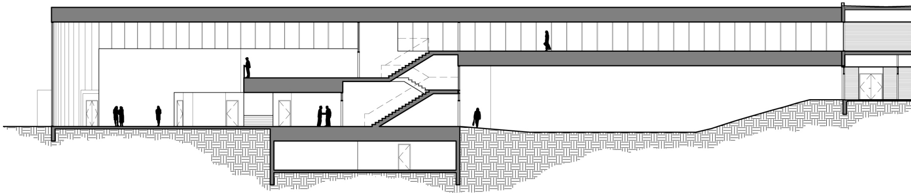
1 NORTH/SOUTH SECTION AT CONNECTING BRIDGE 1/16" = 1'-0"
